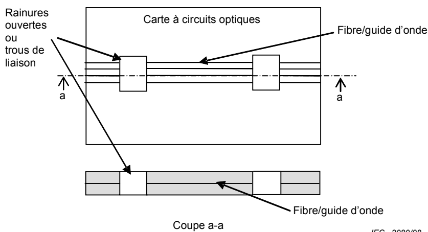
Figure 6 – Configuration D-1
