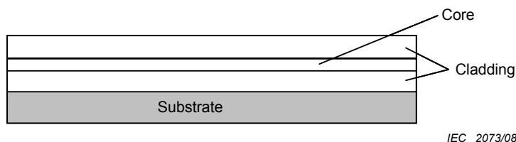
Figure 1a – Example of slab waveguide circuit board
