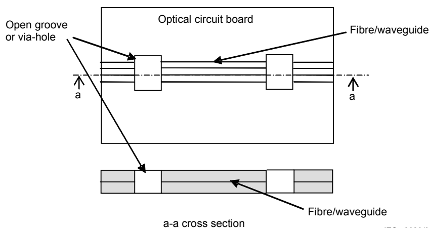
Figure 6 – Configuration D-1
