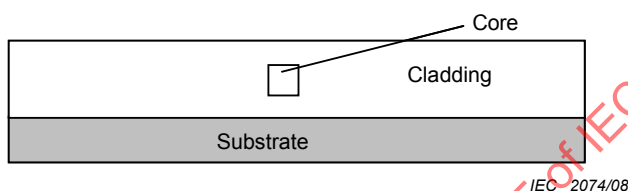
Figure 1b – Example of channel waveguide circuit board – Embedded type
