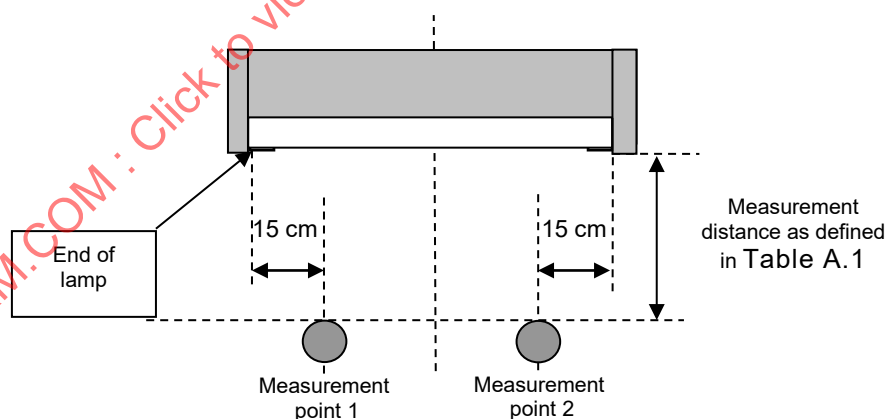
Figure B.1 – Location of measurement point in the transverse direction of lighting equipment – side view
