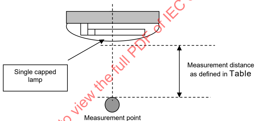
Figure B.3 – Location of measurement points in the longitudinal direction of lighting equipment; in the direction of illumination
