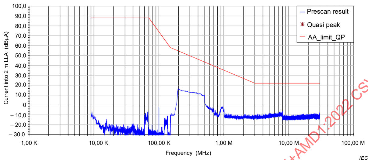
Figure D.5 – Example of magnetic-field test result using the LLA
