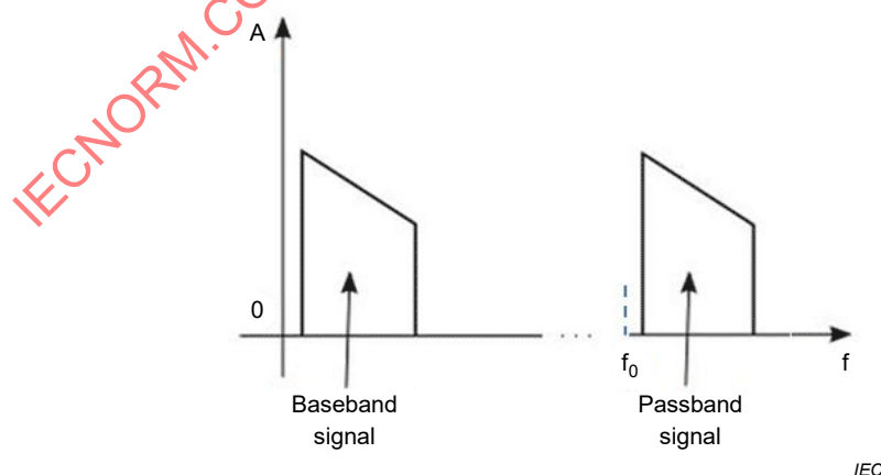
Figure B.2 – Baseband and pass band signals correspondence in SSB modulation
