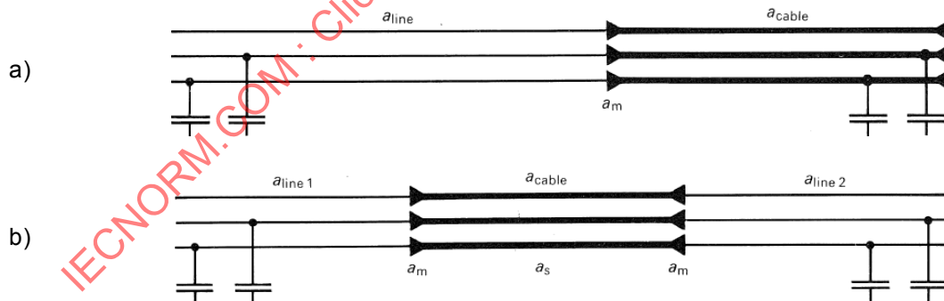
Figure 36 – Junctions of overhead lines with power cables
