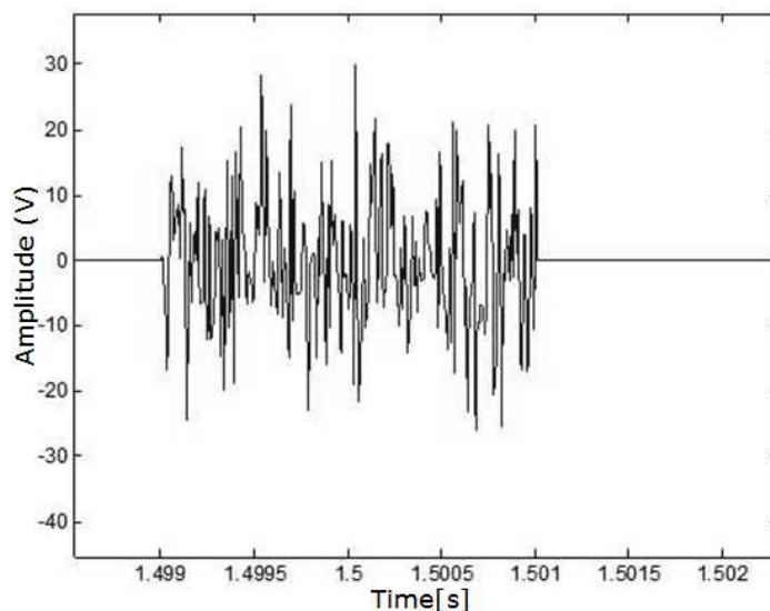
Figure 46 – Burst pulses
