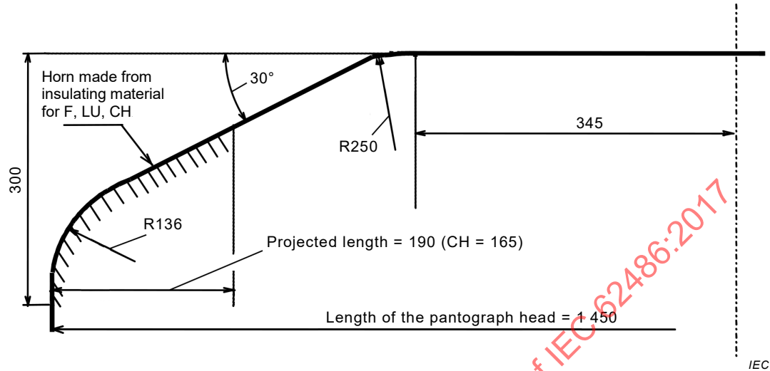
Figure B.1 – Pantograph head with length of 1 450 mm
