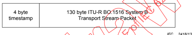
Figure 4 – ITU-R Rec. BO.1516 SYSTEM B Transport Stream Packet with TTS support
