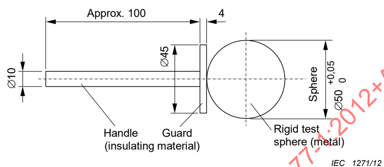
Figure M.1 – Sphere 50 mm probe (IPXXA)
