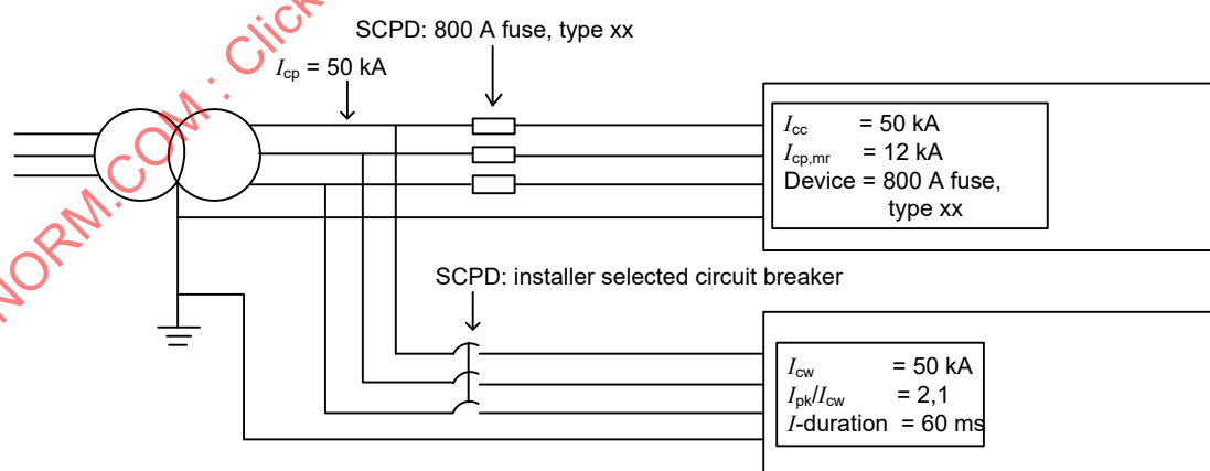
Figure N.5 – Two PECS with different specifications
