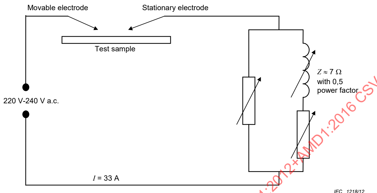
Figure 13 – Circuit for high-current arcing test
