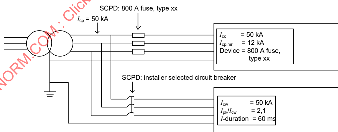
Figure N.5 – Two PECS with different specifications
