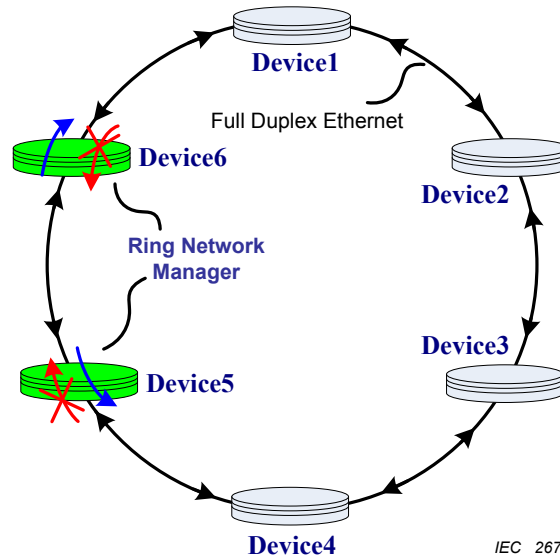
Figure 11 – Ring topology
