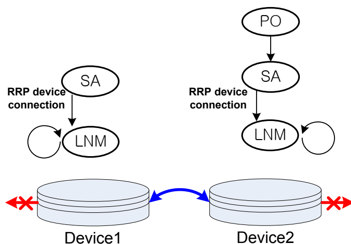
Figure 7 – Devices operation in line network establishing phase
