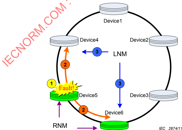
Figure 14 – Device fault on a RNM
