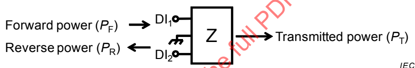
Figure C.2 – Differential DI
