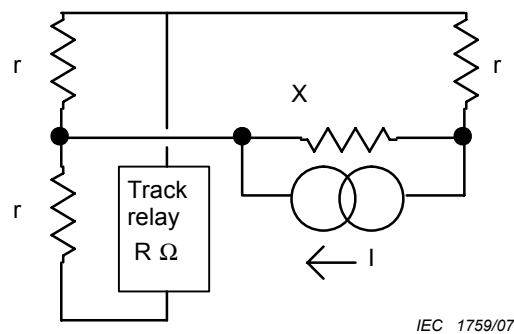
Figure A.9 – Equivalent circuit for Figure A.8
