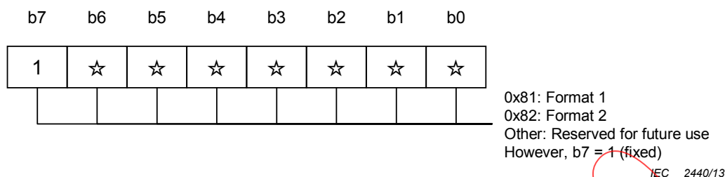
Figure 33 – Detailed specifications of ELHD2
