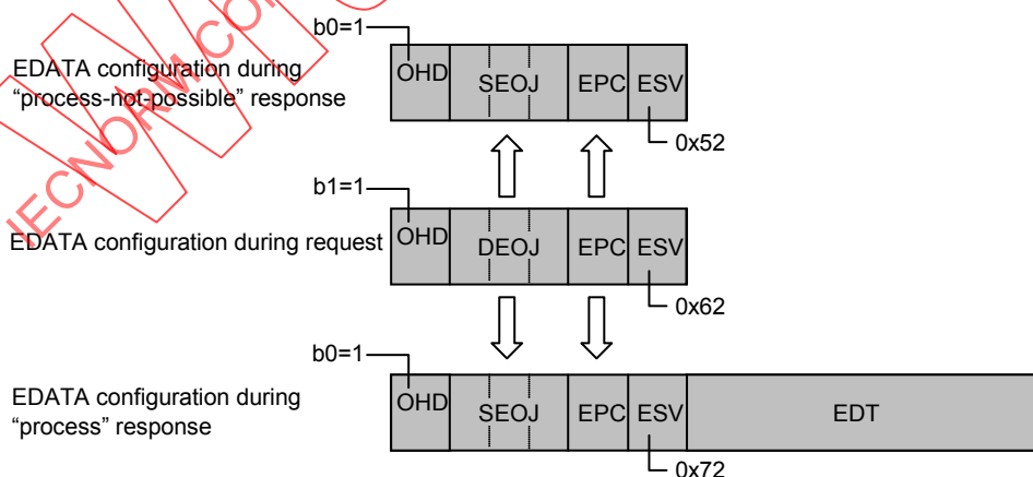
Figure 12 – EDATA configuration in property value read service
