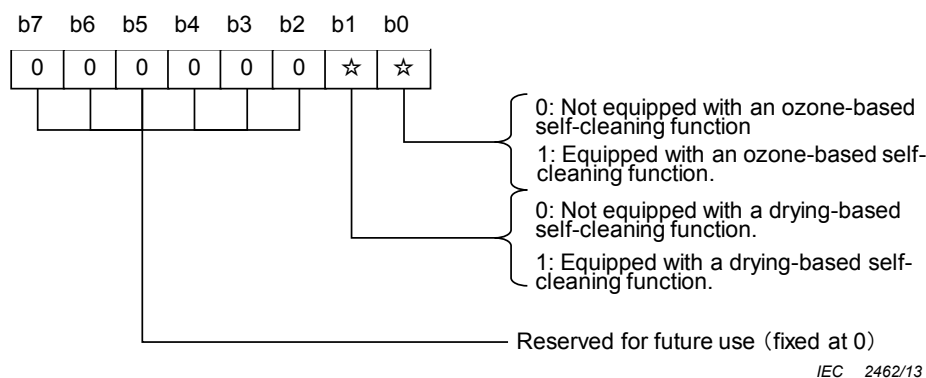
Figure 55 – Self-cleaning method
