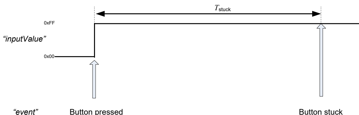
Figure 6 – Button stuck event
