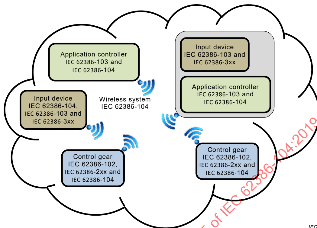
Figure D.2 – Example of an architecture with multiple application controllers
