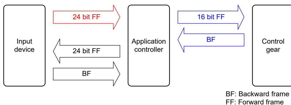
Figure 3 – Communication between bus units (example)
