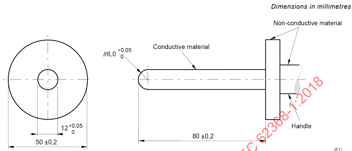
Figure V.3 – Blunt probe
