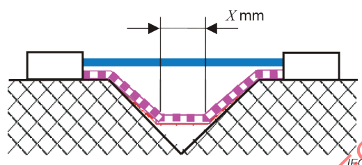
Figure O.2 – Wide groove
