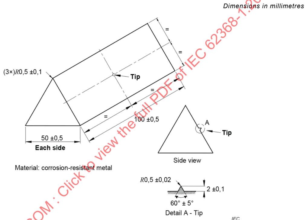
Figure 25 – Mandrel
