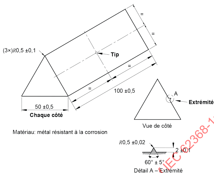
Figure 25 – Mandrin
