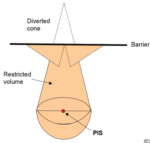
Figure 39b – Illustration showing a horizontal barrier
