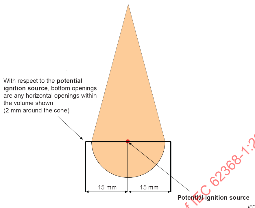
Figure 42 – Bottom openings
