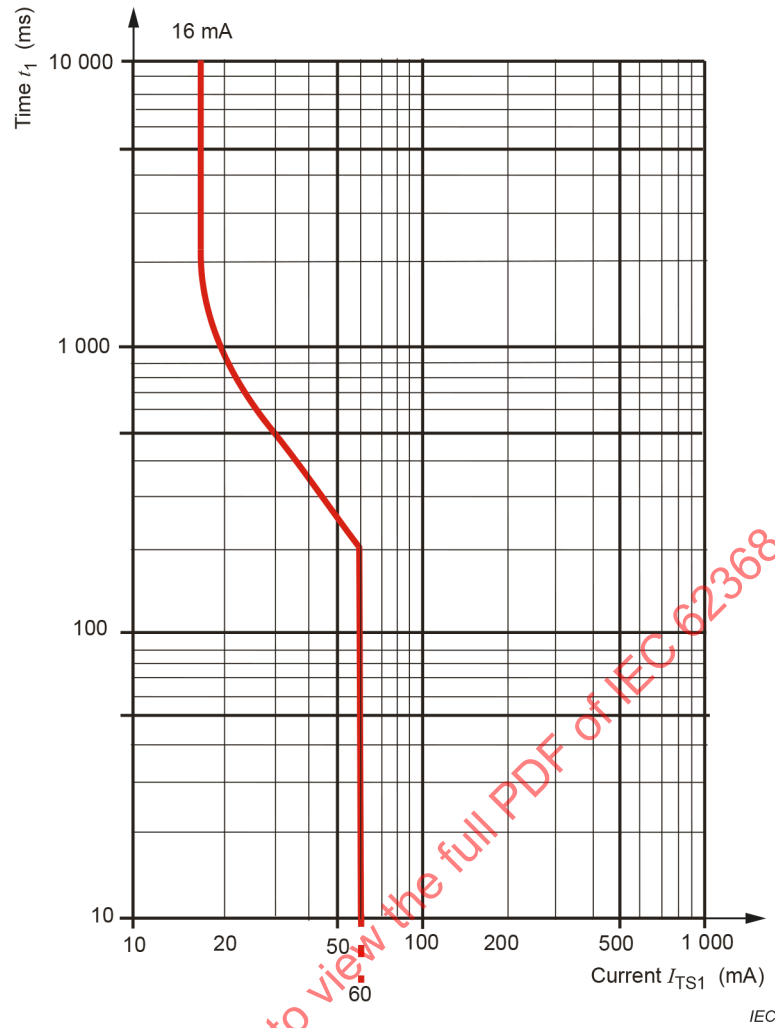
Figure H.2 – I_{TS1} limit curve for cadenced ringing signal
