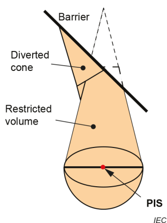
Figure 39a – Illustration showing an angled barrier
