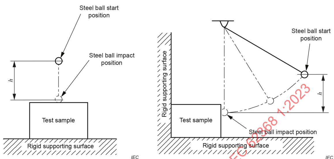
Figure T.1 – Impact test using sphere
