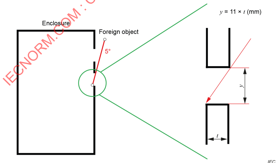
Figure P.3 – Enclosure thickness Safeguards against the consequences of entry of a foreign object
