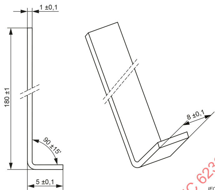
Figure 20 – Test hook
