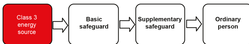
Figure 12 – Model for protection of an ordinary person against a class 3 energy source
