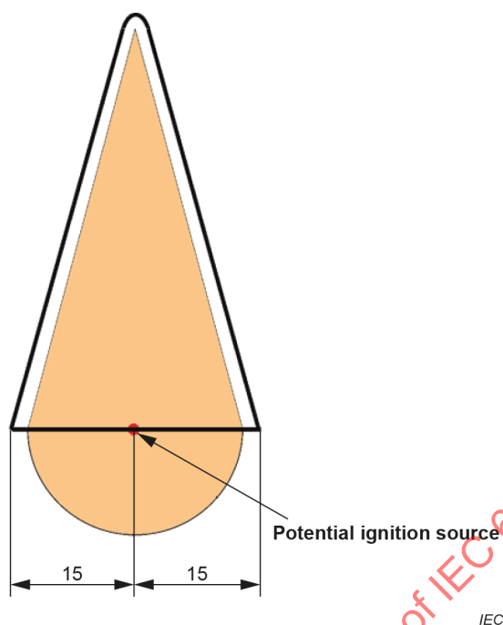
Figure 41 – Top openings
