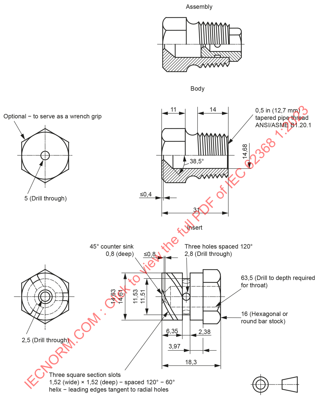
Figure Y.3 – Water-spray test spray head
