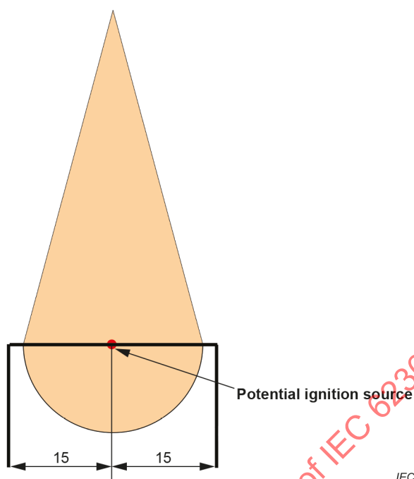
Figure 42 – Bottom openings
