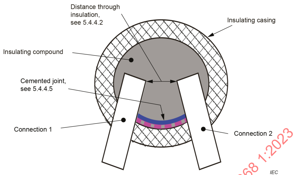
Figure O.15 – Device filled with insulating compound
