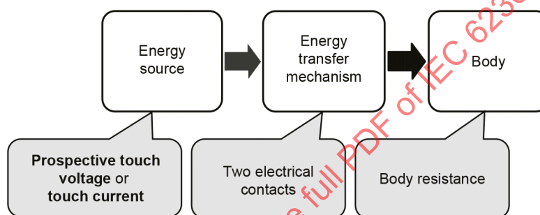
Figure 3 – Schematic and model for electrically-caused pain or injury
