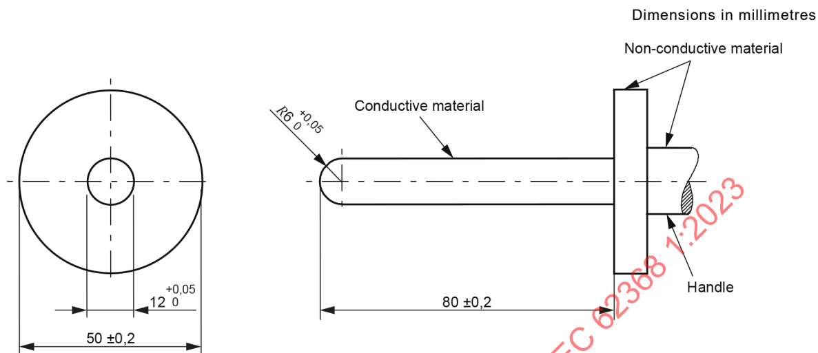
Figure V.3 – Blunt probe
