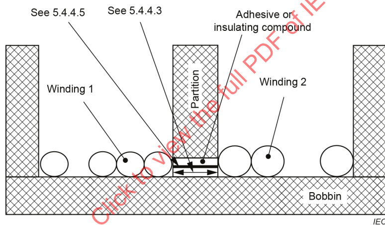
Figure O.16 – Partitioned bobbin
