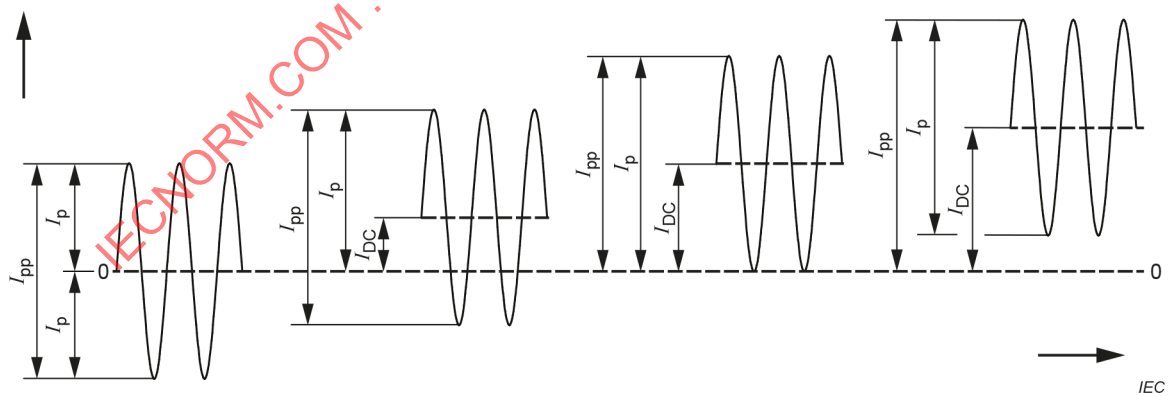
Figure H.3 – Peak and peak-to-peak currents
