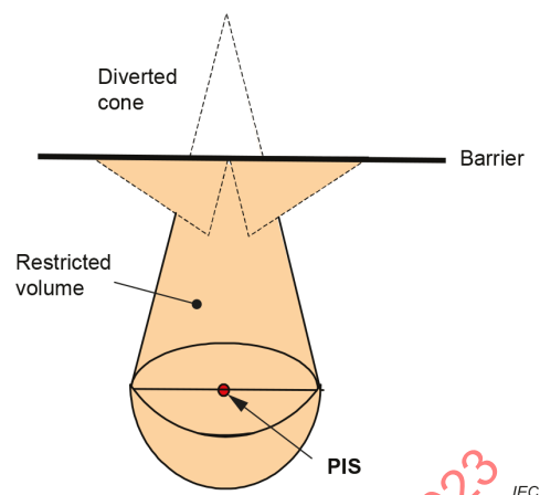
Figure 39b – Illustration showing a horizontal barrier
