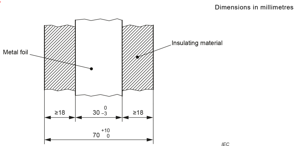
Figure 28 – Position of metal foil on insulating material
