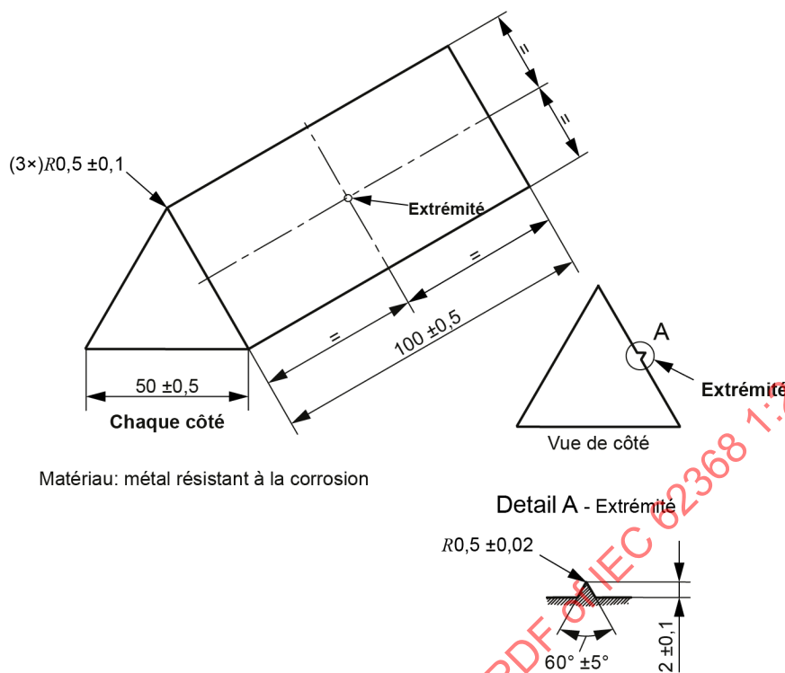
Figure 25 – Mandrin
