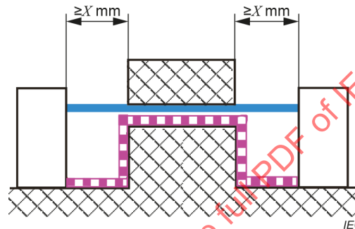
Figure O.6 – Uncemented joint with narrow groove
