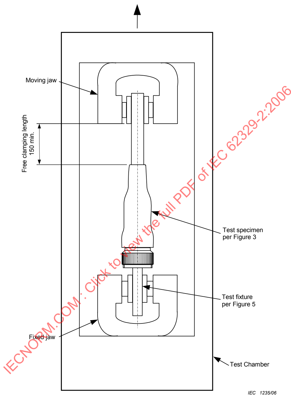
Figure 6 – Test arrangement for dynamic shear
