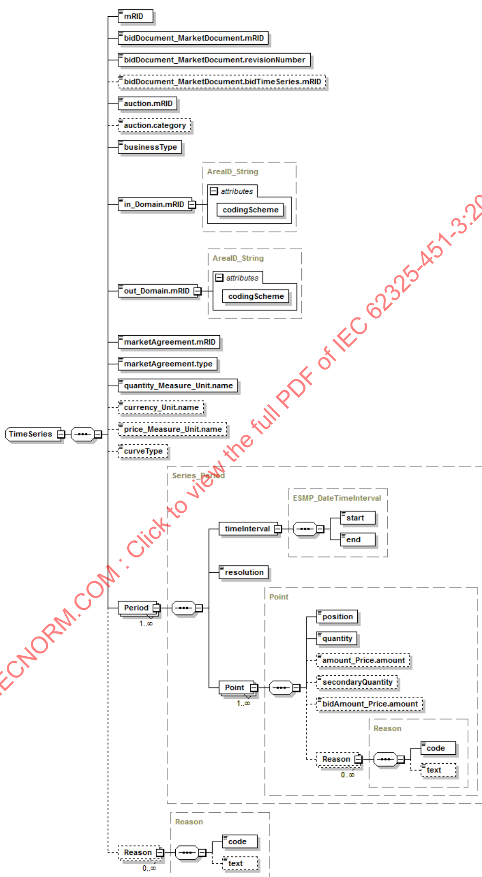
Figure 32 – AllocationResult_MarketDocument XML schema structure – 2/2
