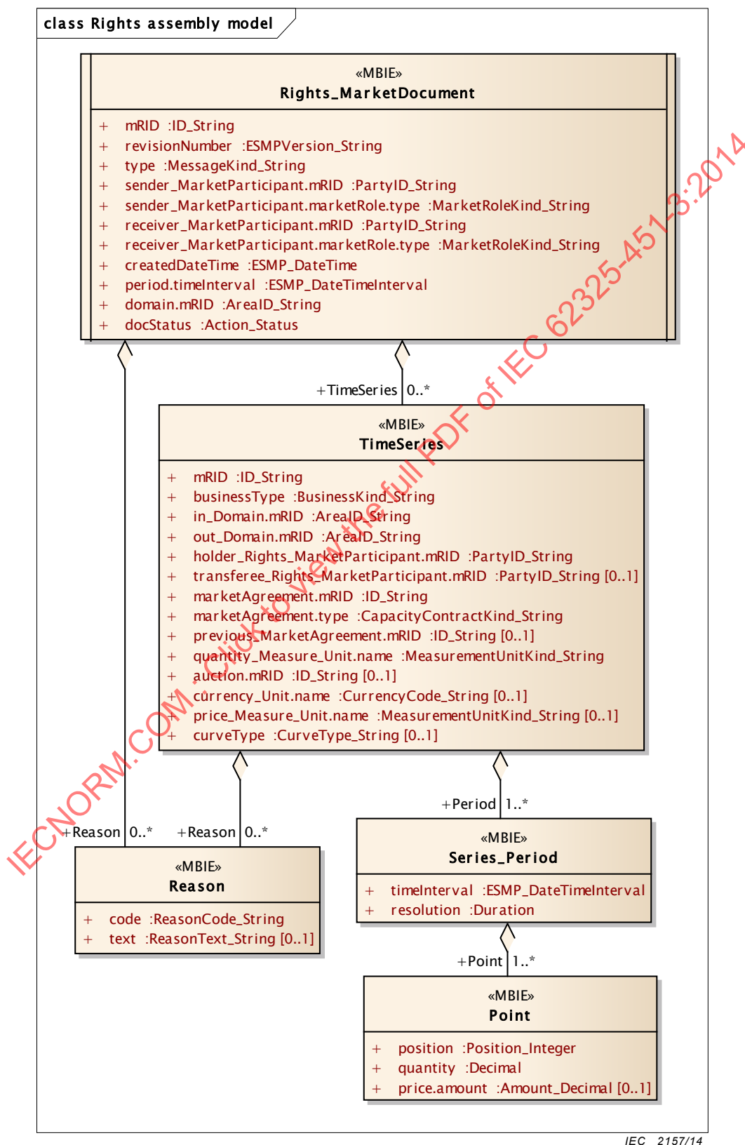
Figure 24 – Rights assembly model
