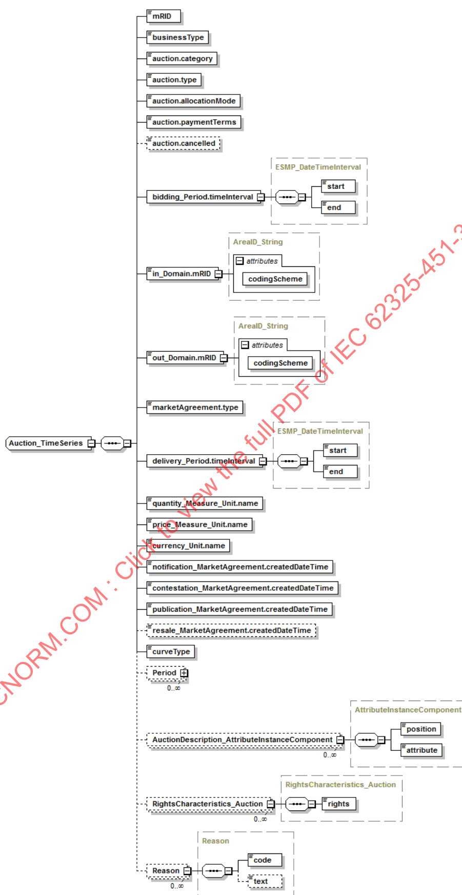
Figure 28 – CapacityAuctionSpecification_MarketDocument XML schema structure – 2/2
