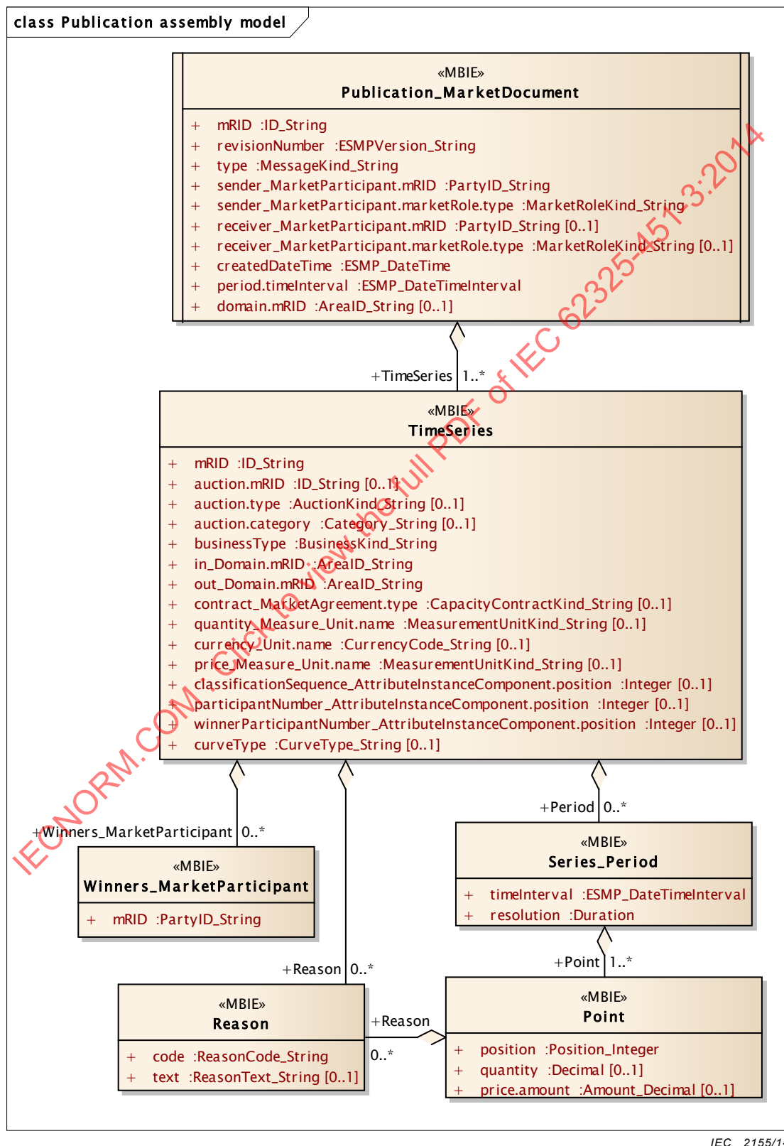
Figure 22 – Publication assembly model
