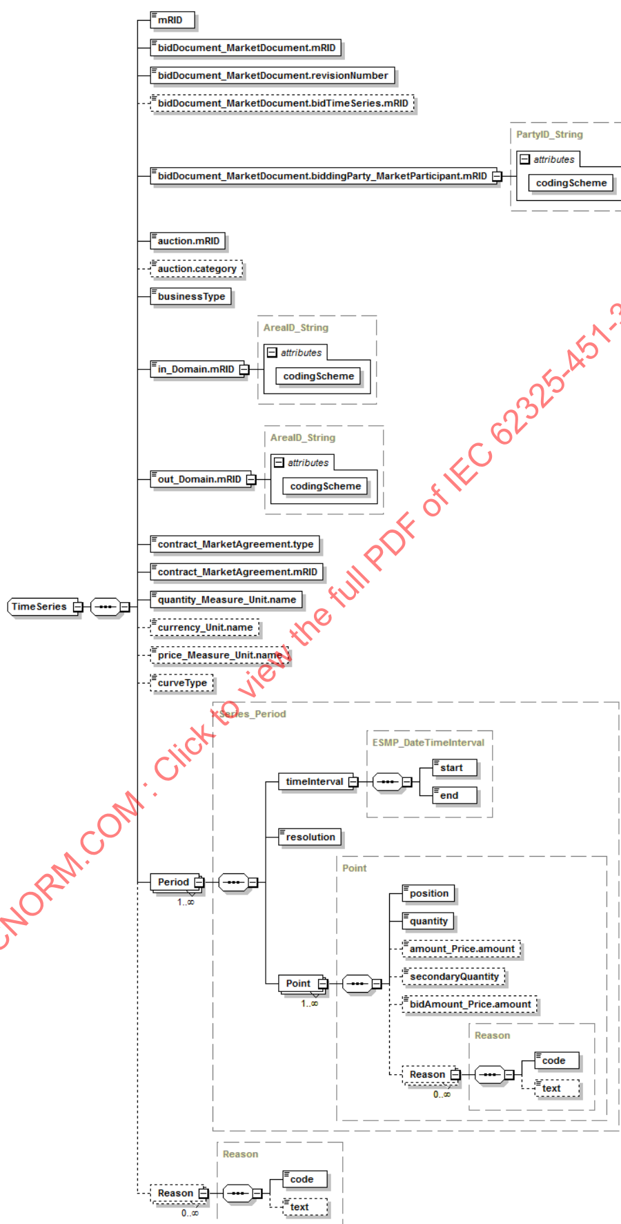
Figure 34 – TotalAllocationResult MarketDocument XML schema structure – 2/2
