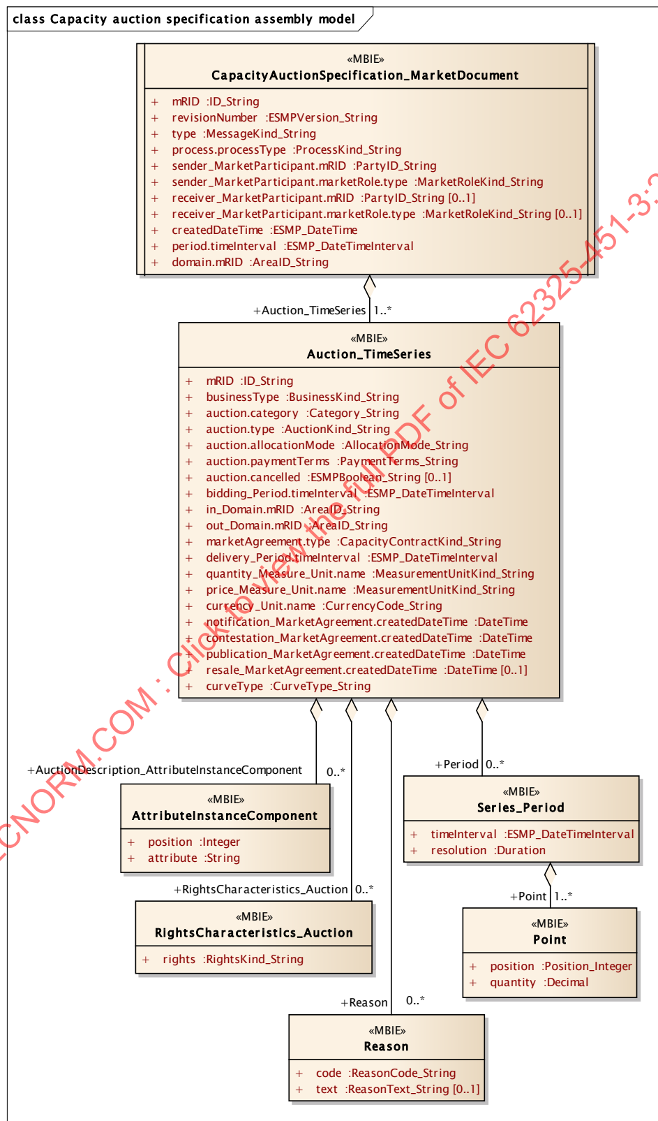
Figure 12 – Capacity auction specification assembly model
