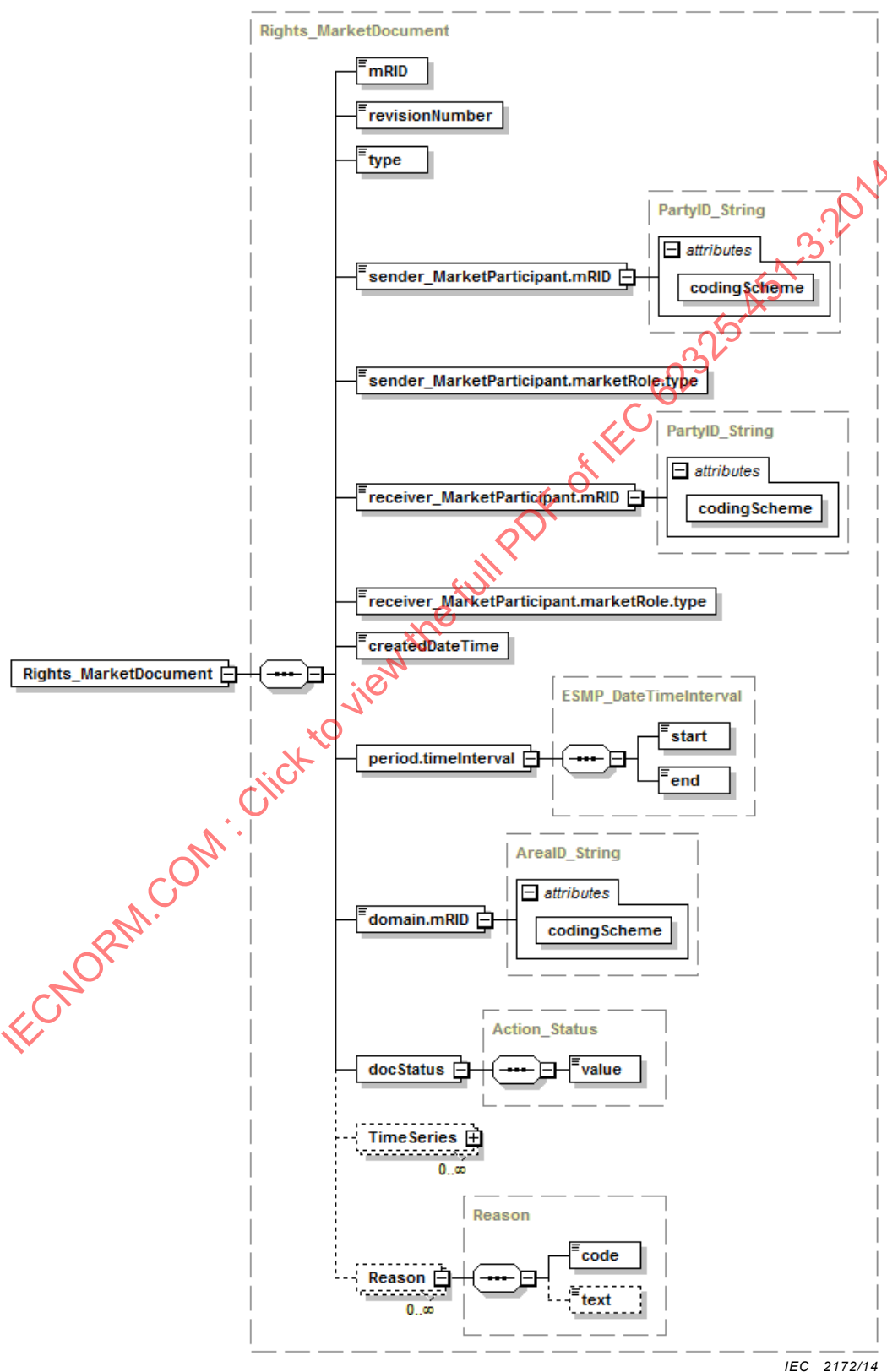
Figure 39 – Rights_MarketDocument XML schema structure – 1/2
