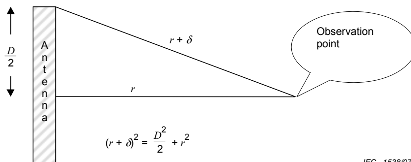
Figure A.1 – Geometry of antenna with largest linear dimension D
