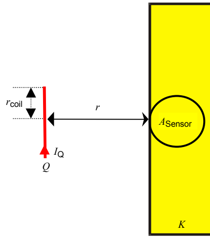
Figure C.15 – Position of source Q , sensor and model K
