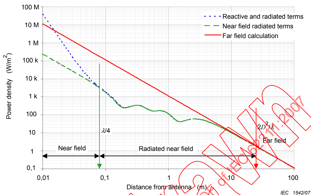
Figure A.5 – Far-field = straight line, radiated near-field = lower line & all near-fields = other line
