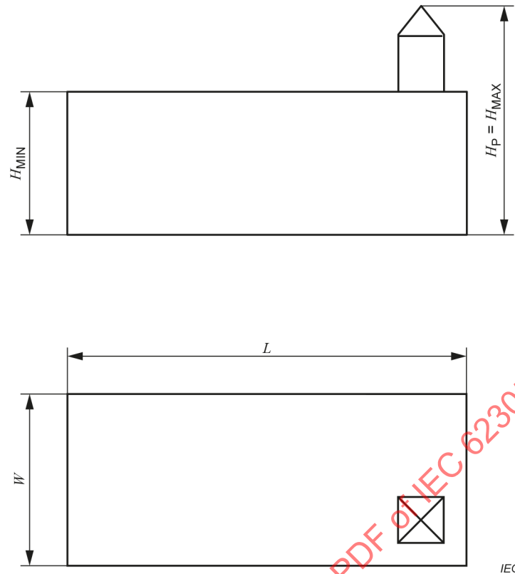
Figure A.2 – Structure de forme complexe
