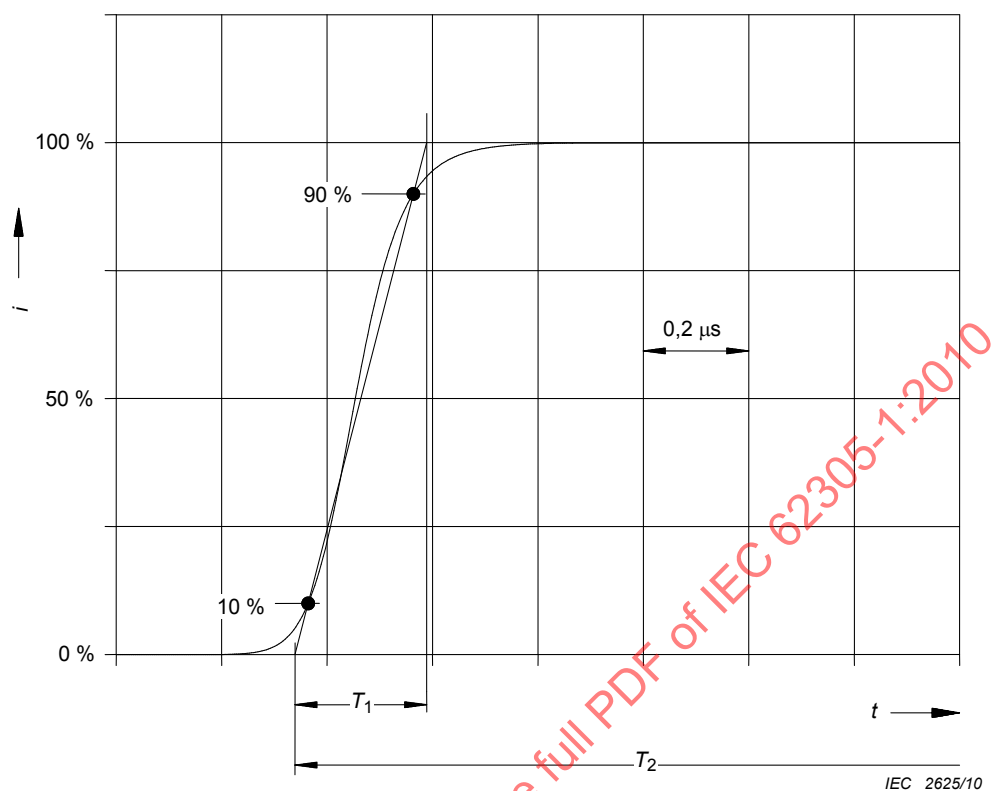
Figure B.5 – Shape of the current rise of the subsequent negative impulses
