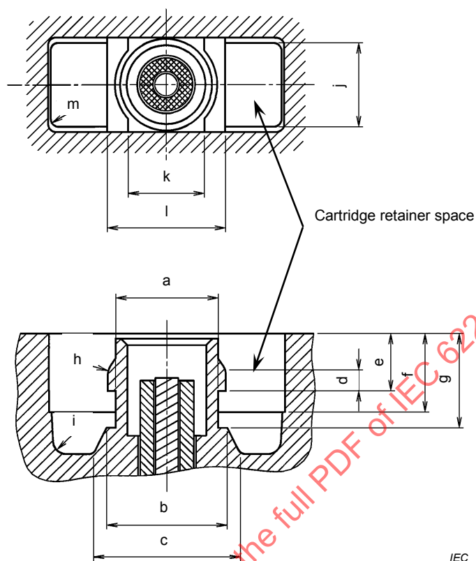
Figure 41 – Connector retainer
