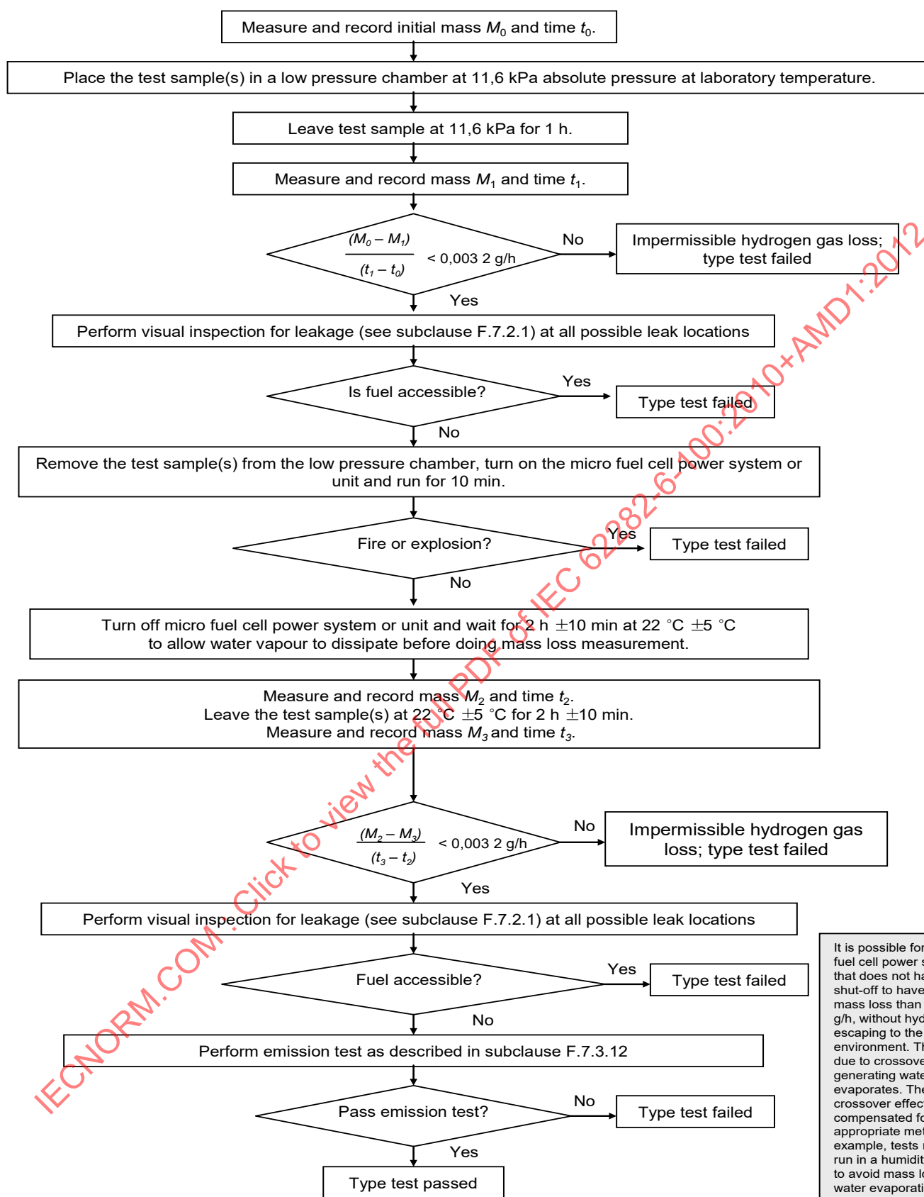
Figure F.7 – Micro fuel cell power system or micro fuel cell power unit leakage and hydrogen gas loss test flow chart for 11,6 kPa low external pressure test – Replaces Figure 7
