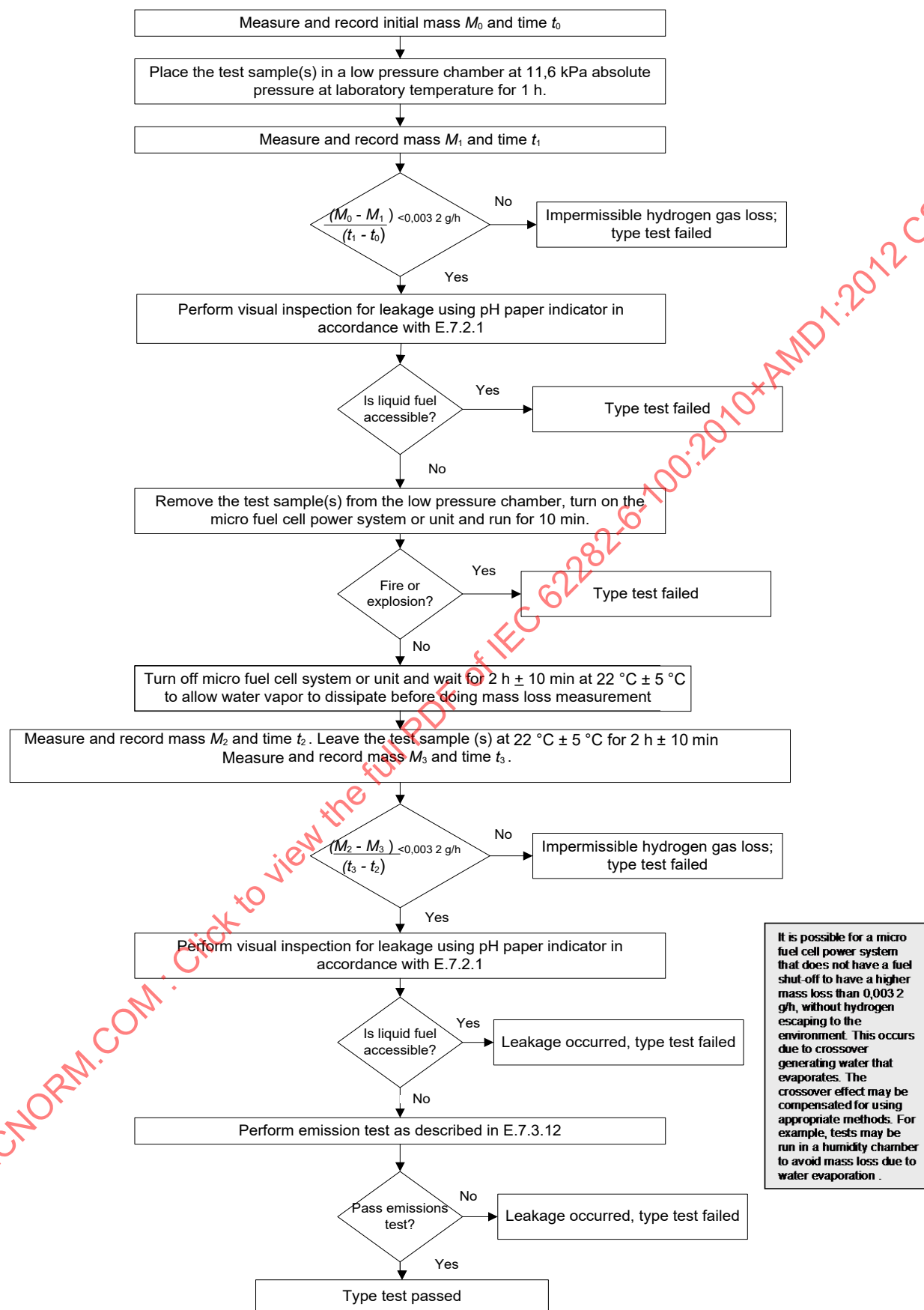
Figure E.7 – Micro fuel cell power system or micro fuel cell power unit leakage and hydrogen gas loss test flow chart for 11,6 kPa low external pressure test – Replaces Figure 7
