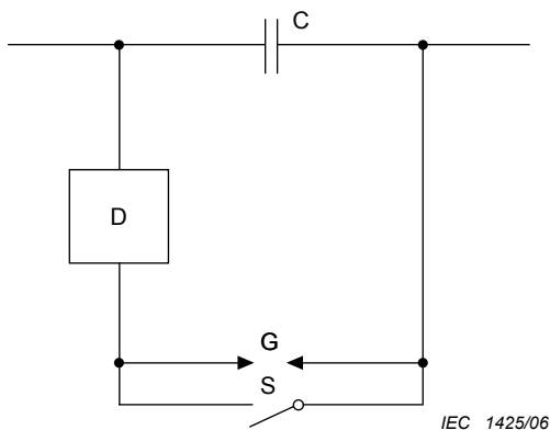
Single gap
