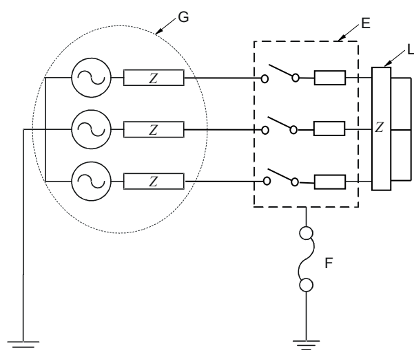
Figure 2a – Test circuit with load
