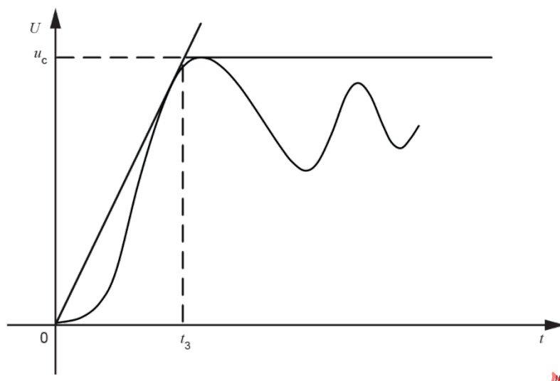
Figure 4 – Example of a two parameters envelope for a TRV
