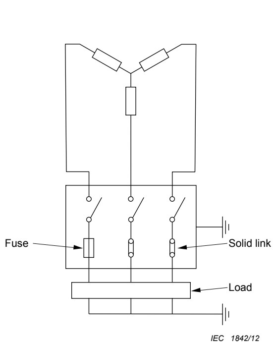
Figure 2a – Preferred earth point
