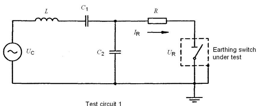
Test circuit 1
