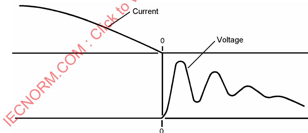
Figure F.2 – TRV in case of ideal breaking
