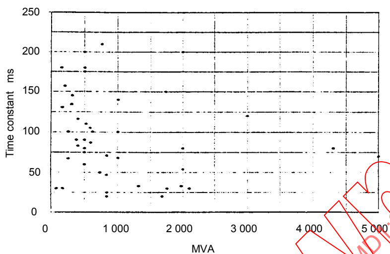
Figure 1 – Typical short-circuit testing station parameter combinations
