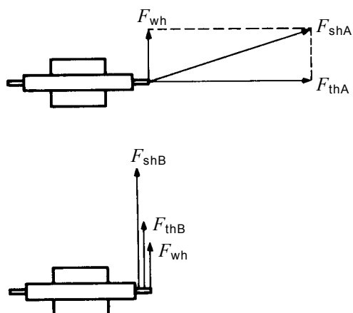
Horizontal forces
