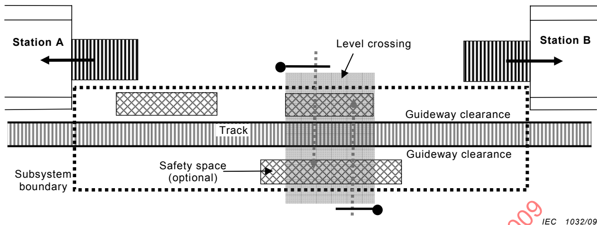
Figure 4 – Boundary of the “guideway between stations” subsystem with level crossing
