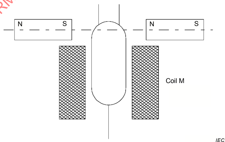
Figure B.2 – Test system 2
