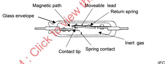
Figure 2 – Example of heavy-duty reed switch structure
