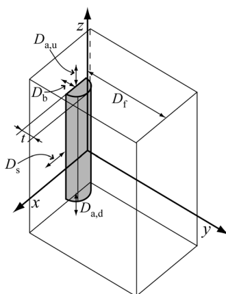
Figure C.3 – Example of parallelepipedic compliance boundary
