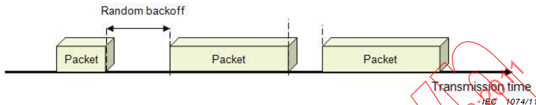
Figure N.4 – Example of Wi-Fi frames
