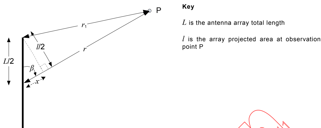
Figure B.3 – Maximum path difference for an antenna with largest linear dimension L
