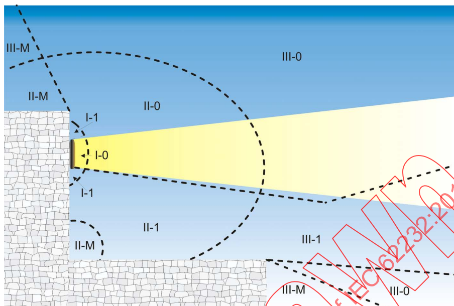
Figure B.4 – Example source-environment plane regions near a roof-top antenna which has a narrow vertical (elevation plane) beamwidth (not to scale)
