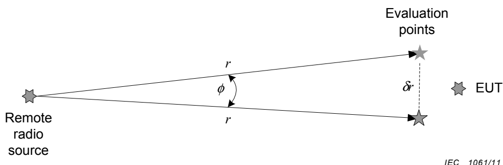
Figure K.2 – Relationship of separation of remote radio source and evaluation area to separation of evaluation points
