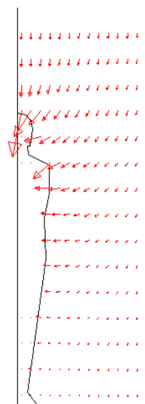
Figure 14 – Mesh of the man body model and distortion of power frequency electric field lines close to model
