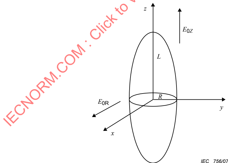
Figure 7 – Conductive spheroid exposed to electric field
