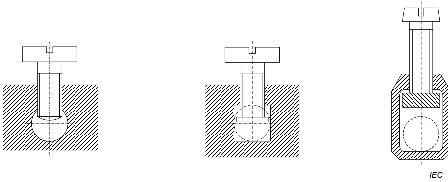
Figure 9a – Pillar terminals
