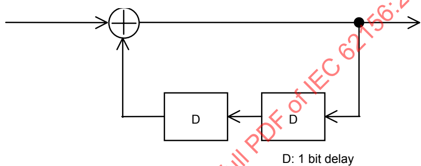
Figure 24 – Pre-coding
