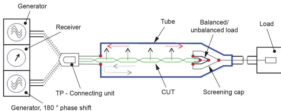
Figure D.3 – Configuration for near end coupling measurement of an unscreened single pair, principle set-up
