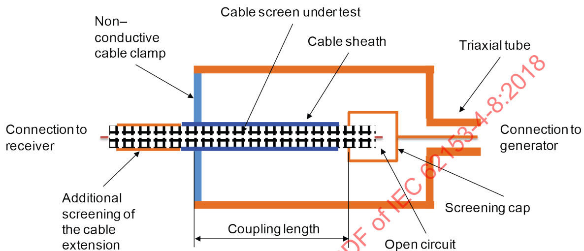
Figure 5 – Triaxial set-up
