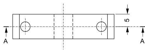
Figure 5 – Impedance matching part of launcher – Position 3
