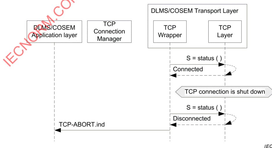
Figure A.4 – Polling the TCP sublayer for TCP abort indication
