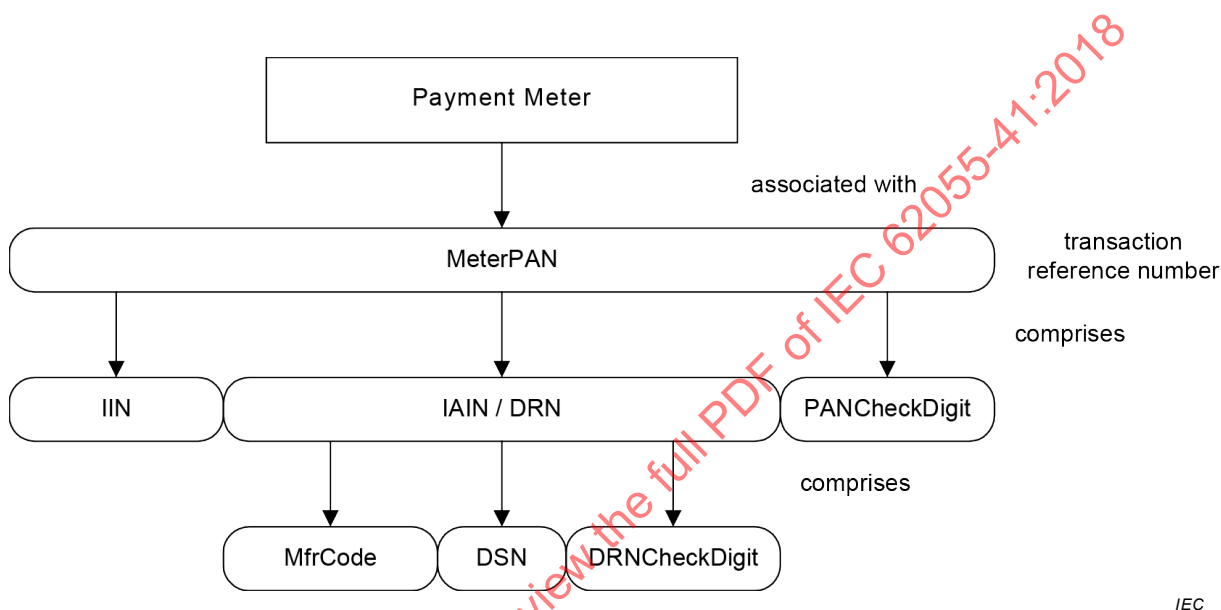
Figure 5 – Composition of transaction reference number
