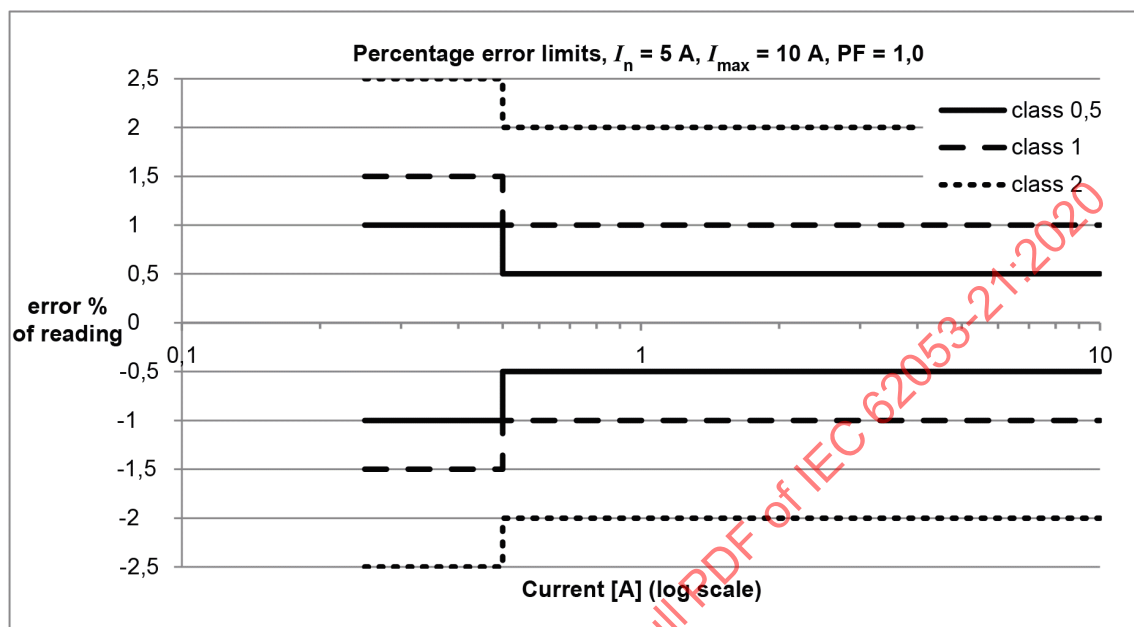
Figure A.1 – Comparison of acceptable percentage error limits for meters of classes 0,5, 1 and 2, with I_n = 5 \text{ A} and I_{\max} = 10 \text{ A} , at \text{PF} = 1,0 , for direct connection
