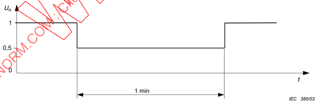
Figure B.3 – Voltage dips of \Delta U = 50 \%
