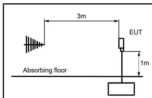
Figure E.1 – Test set-up for the test of immunity to electromagnetic RF fields
