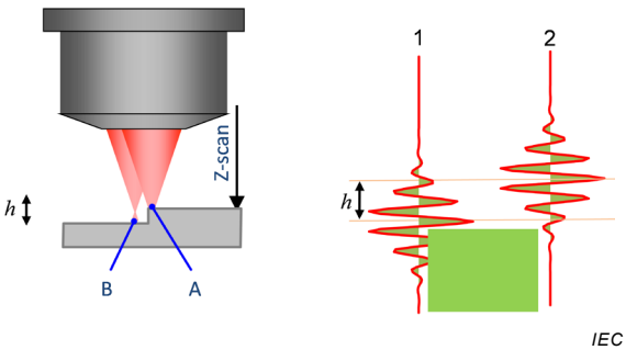
a) Basic features of CSI microscope
