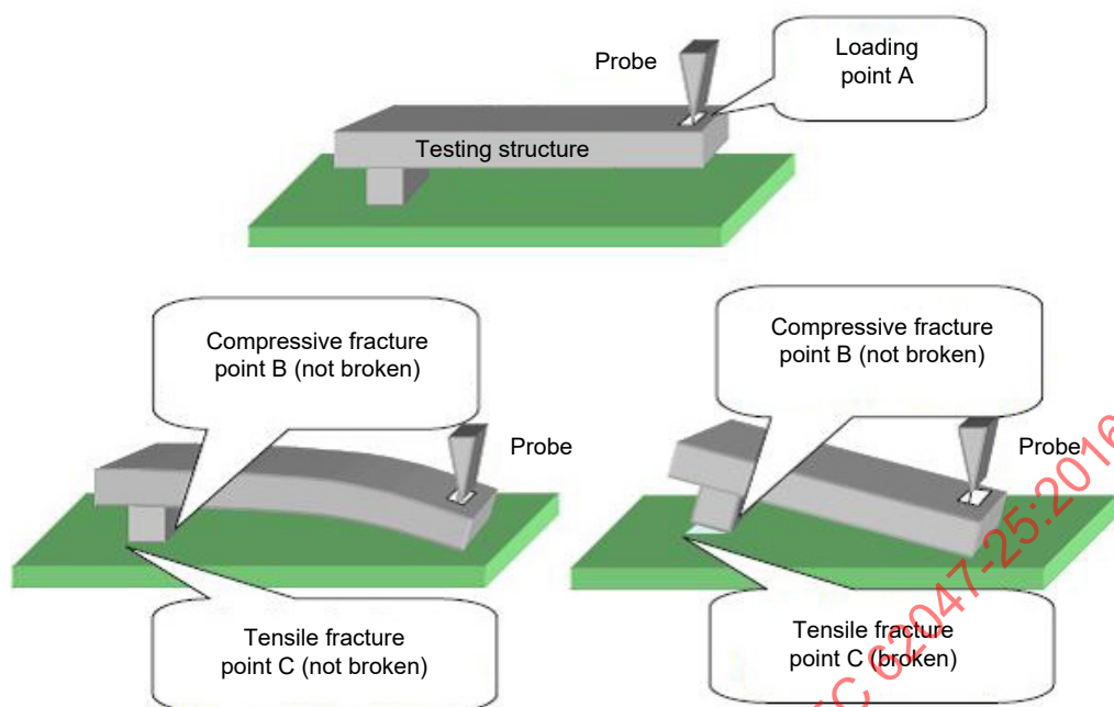
Figure 3 – Pull-press testing method operation process
