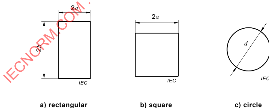
Figure 4 – Bulge membrane window shapes
