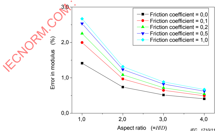
Figure A.1 – Error estimation with the aspect ratio and friction coefficient in the elastic modulus measurement
