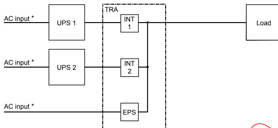
Figure C.12 – Multiple function bypass, interrupter and isolation switch
