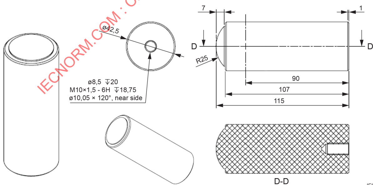
Figure 3 – Hammer description
